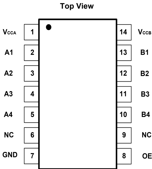
Fig.5-3. GT0104: TD (TSSOP14) Package
