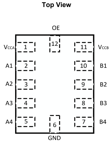
Fig.5-2. GT0104: SC (QFN2.0x2.0-12L) Package
