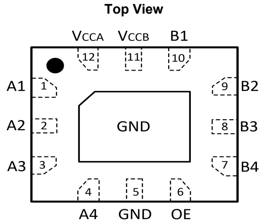
Fig.5-2. GT0104: SC (QFN2.0x2.0-12L) Package
